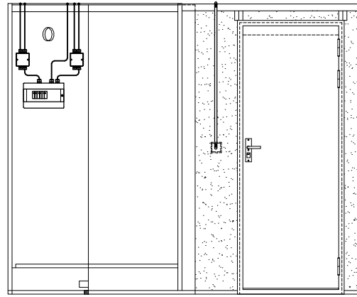
View "E" 1:20
