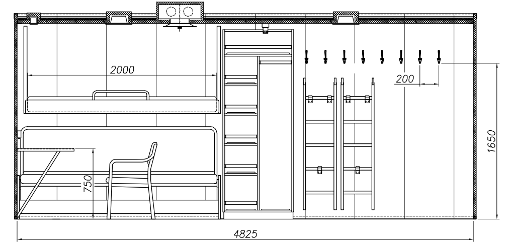
View "A" 1:20
