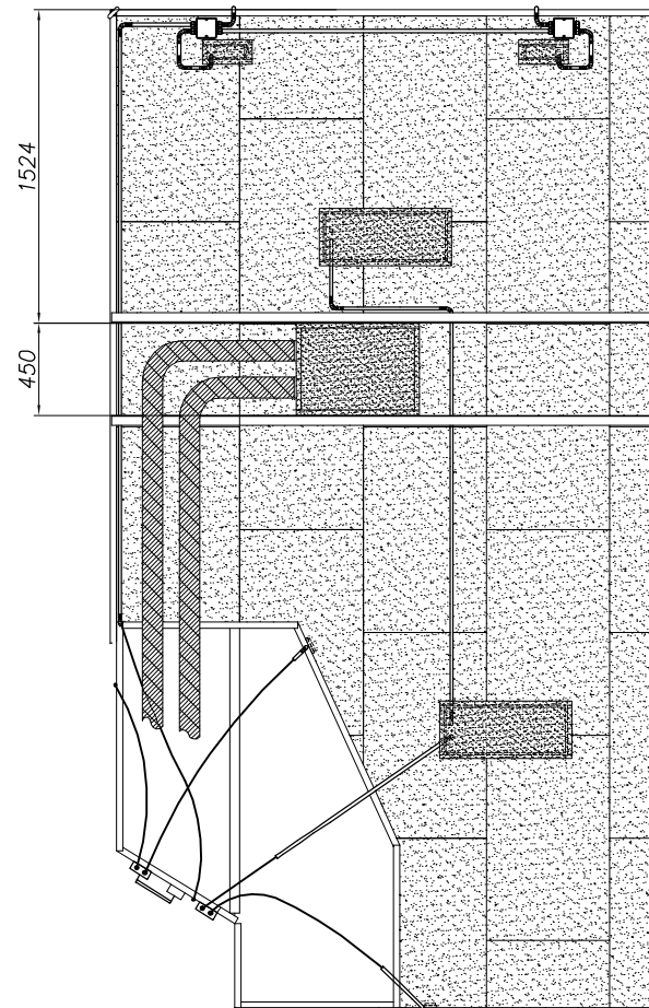
View "F" 1:20
