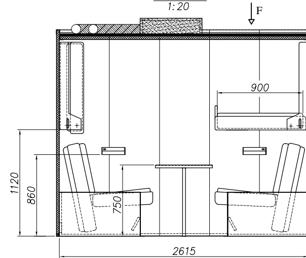
View "A" 1:20
