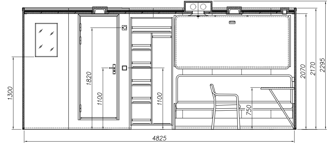
View "D" 1:20
