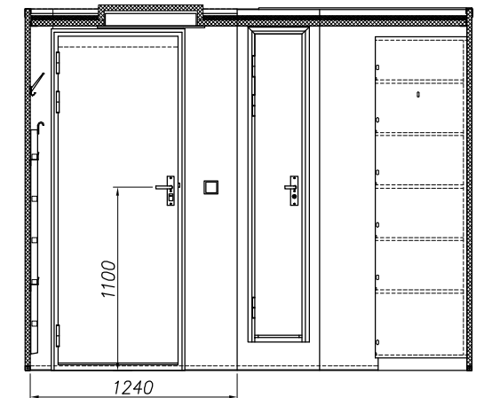
View "C" 1:20
